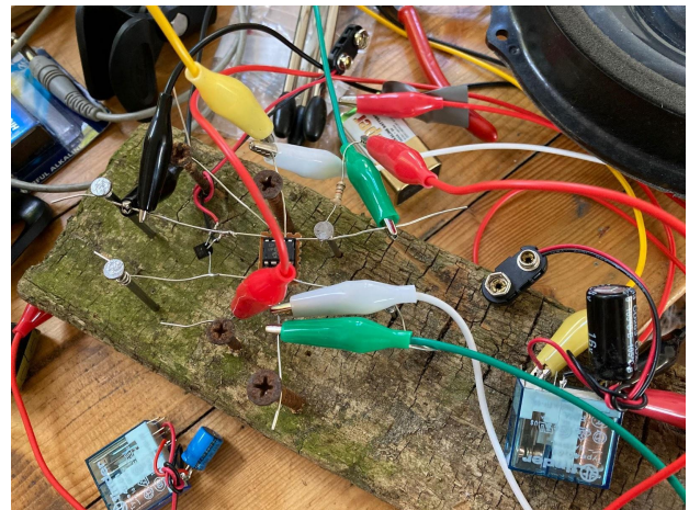
Figure 12. Radical Nails/DAC-less Synth and Clickers (mechanical oscillators made from a relay, capacitor and battery)
