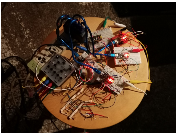
Figure 11. Five different versions of Floating Noise
