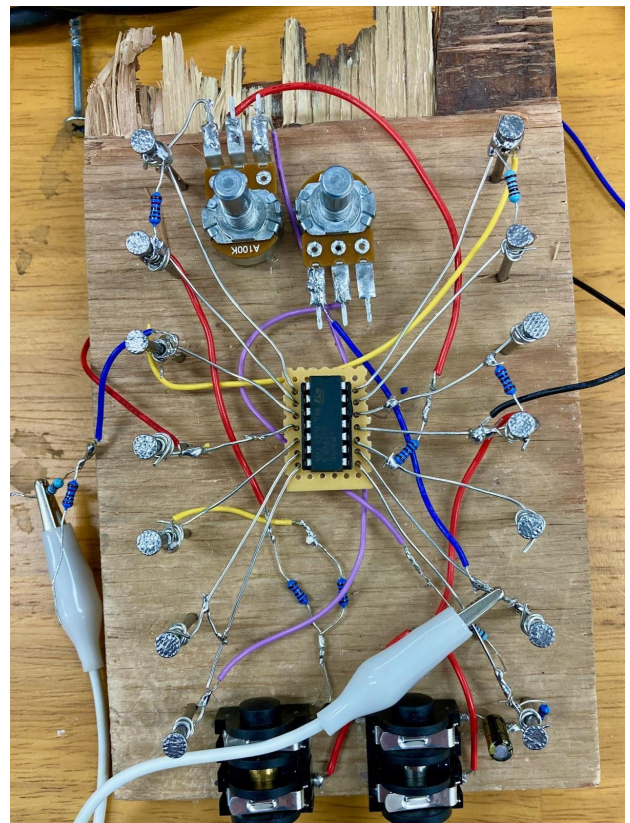
Figure 3. Bad Buffer.
